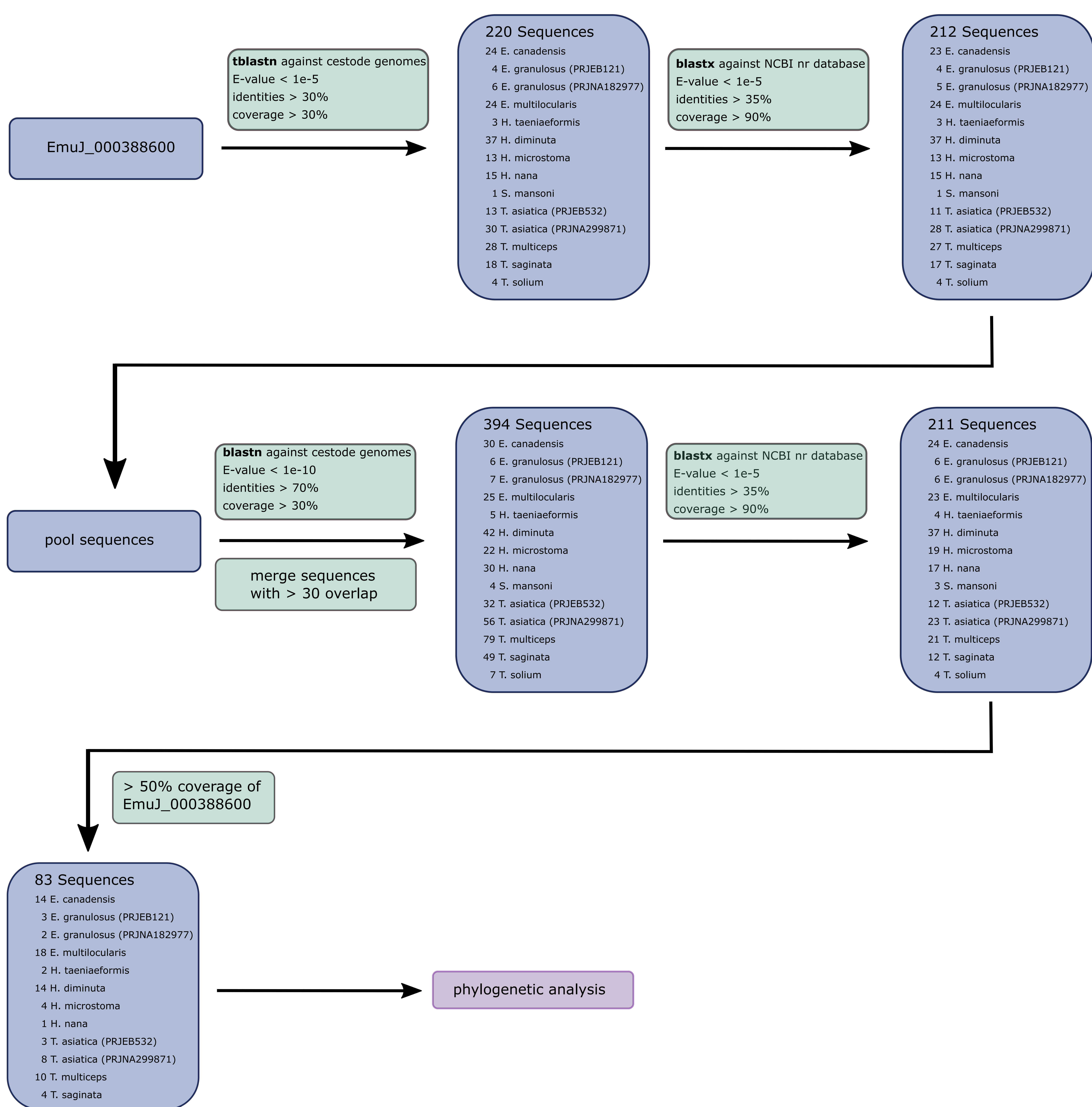
Additional file 2: Figure S1. Schematic overview of the bioinformatic workflow
