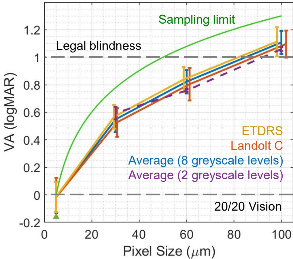
Supp. Figure 1. Single-character visual acuity ( n=13 for 30 and 60 \mu\text{m} pixels; n=19 for natural vision and 100 \mu\text{m} pixels). In addition to the data presented in Figure 3, the results of ETDRS and Landolt C VA are shown separately here. Error bars are presented in terms of s.d.
