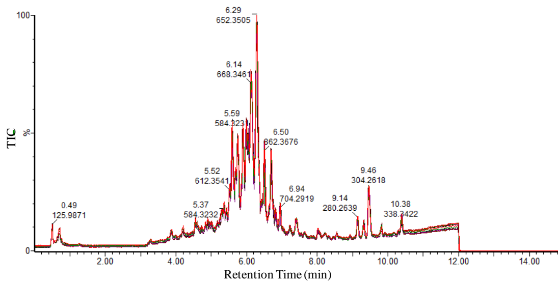
Figure S1 The total ion chromatograms of all the samples.
