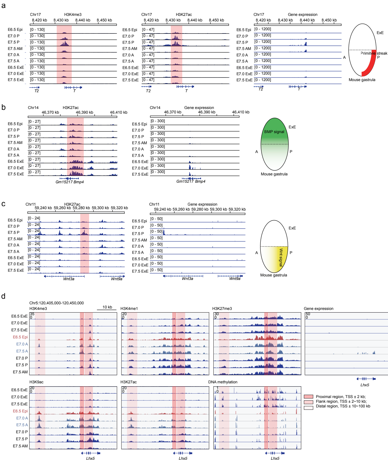
Supplementary information, Fig. S2 The representative genome browser snapshot exhibits epigenetic modification and gene expression changes during mouse gastrulation.
