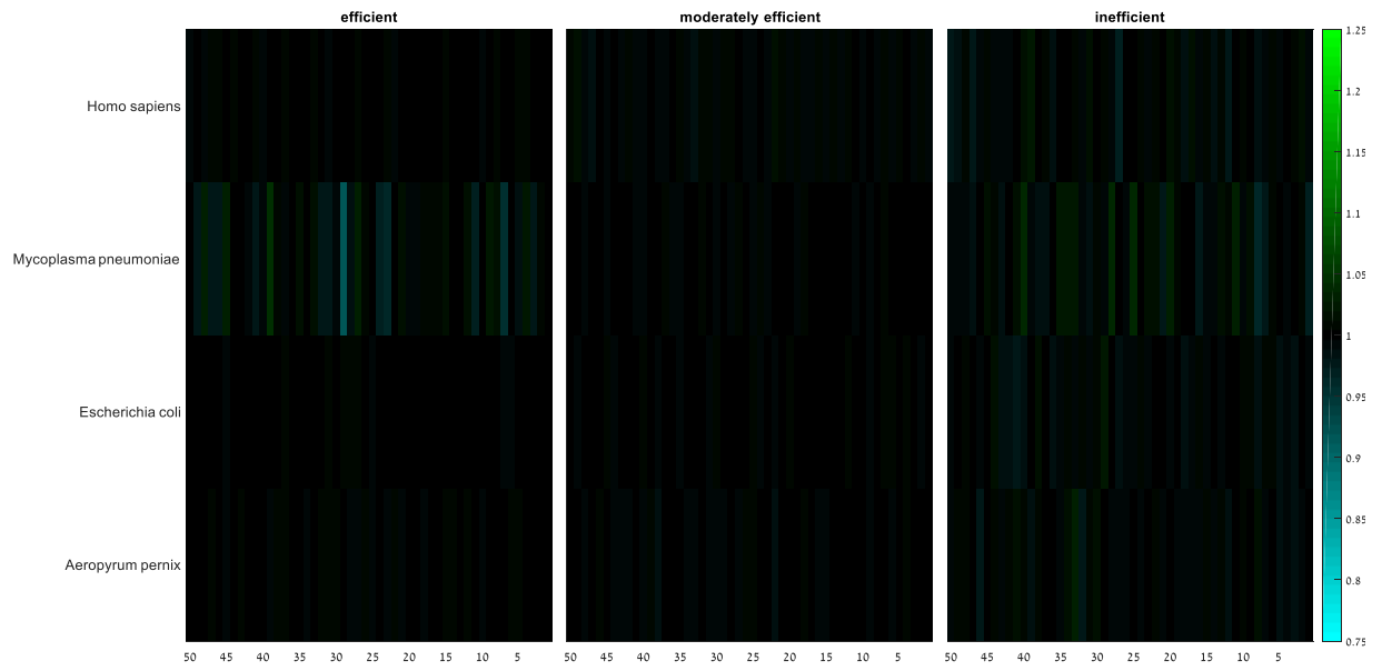
Figure S1. Group RSCA scores ( R_{\alpha}^S ) of efficient, moderately efficient, and inefficient codons along the last 50 codons of the gene for random codon permutation. Rows denote species, columns denote positions.
