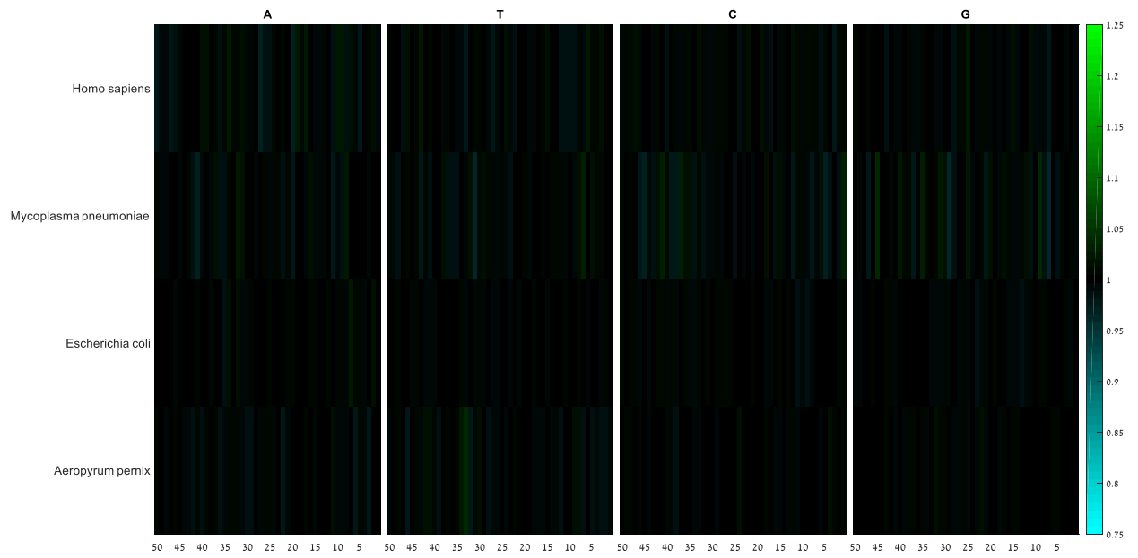
Figure S2. Group RSCA scores ( R_{\alpha}^S ) of A-ending, T-ending, C-ending, and G-ending codons along the last 50 codons of the gene for random codon permutation. Rows denote species, columns denote positions.
