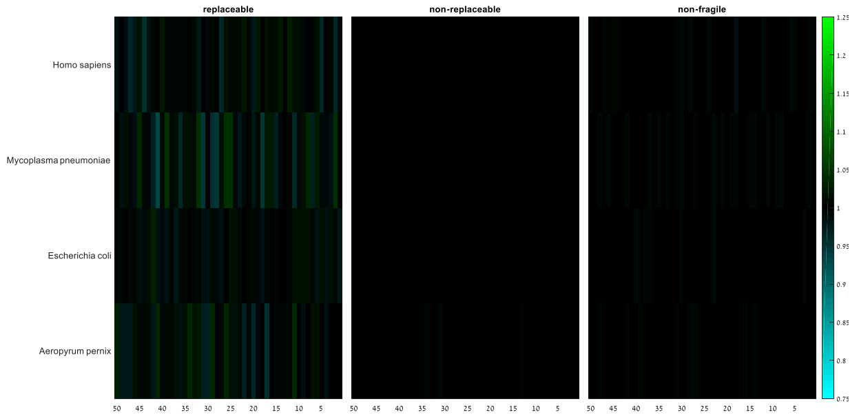
Figure S3. Group RSCA scores ( R_{\alpha}^S ) of replaceable, non-replaceable, and non-fragile codons along the last 50 codons of the gene for random codon permutation. Rows denote species, columns denote positions.
