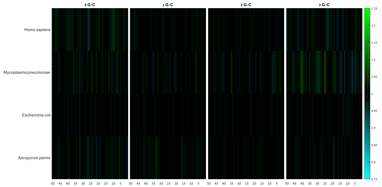
Figure S4. Group RSCA scores ( R_{\alpha}^S ) of 0, 1, 2, and 3 G/C codons along the last 50 codons of the gene for random codon permutation. Rows denote species, columns denote positions.
