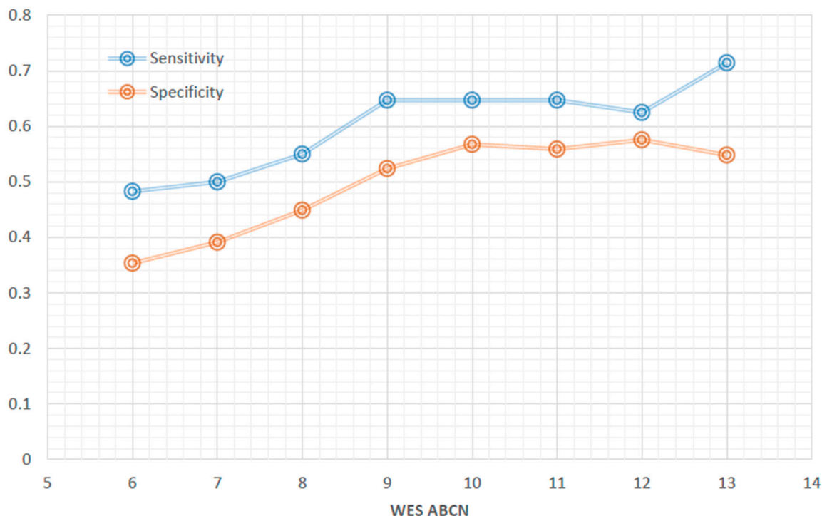
Figure S1. The total sensitivity and specificity curve for absolute copy number based on different WES absolute copy number gain cut-off from 6 to 13.
