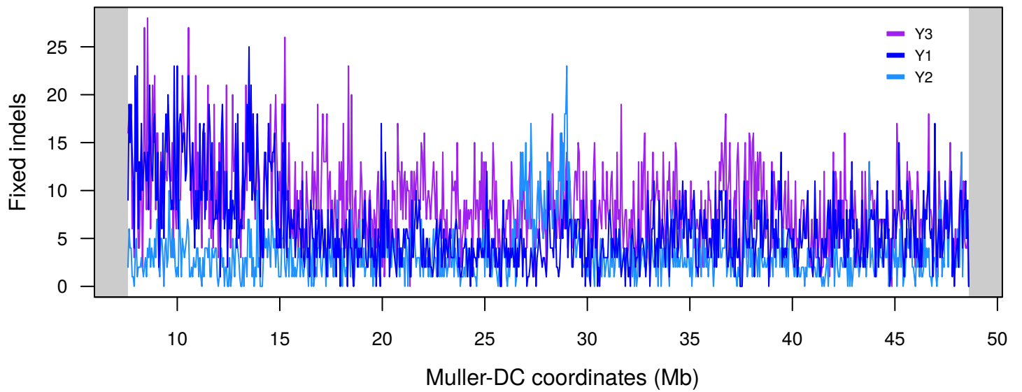
S14 Fig. Distribution of fixed derived SNPs (top) and indels (bottom) on the three neo-Y haplotypes: Y1 (blue), Y2 (light blue), Y3 (purple).
