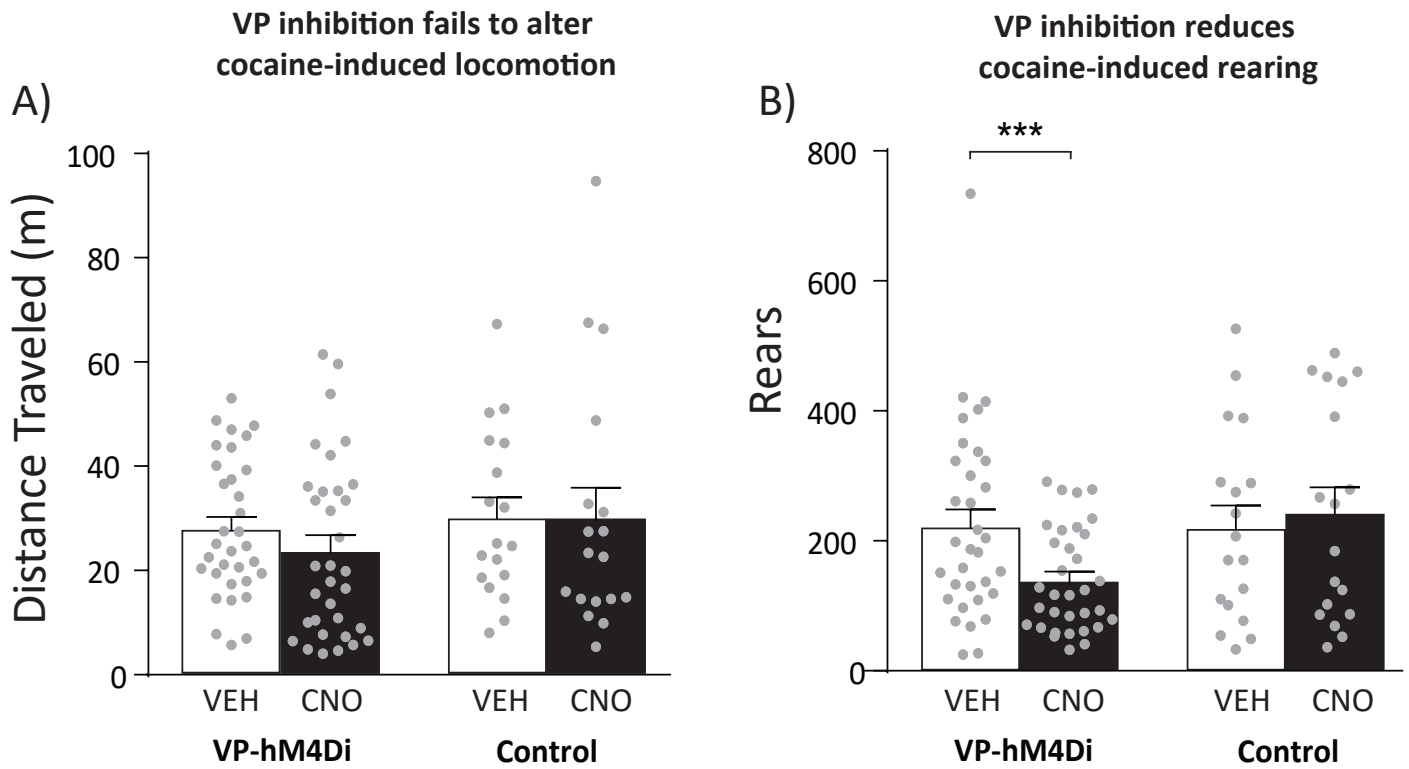
Supplemental Figure 2. VP inhibition decreases cocaine-induced rearing, but not distance traveled. A) Within subjects tests showed that CNO in VP-hM4Di rats and controls fails to alter cocaine-induced horizontal locomotion. B) CNO decreases rearing in VP-hM4Di rats, but not controls. Control = extra-VP hM4Di and eGFP-only rats. *** p < 0.001
