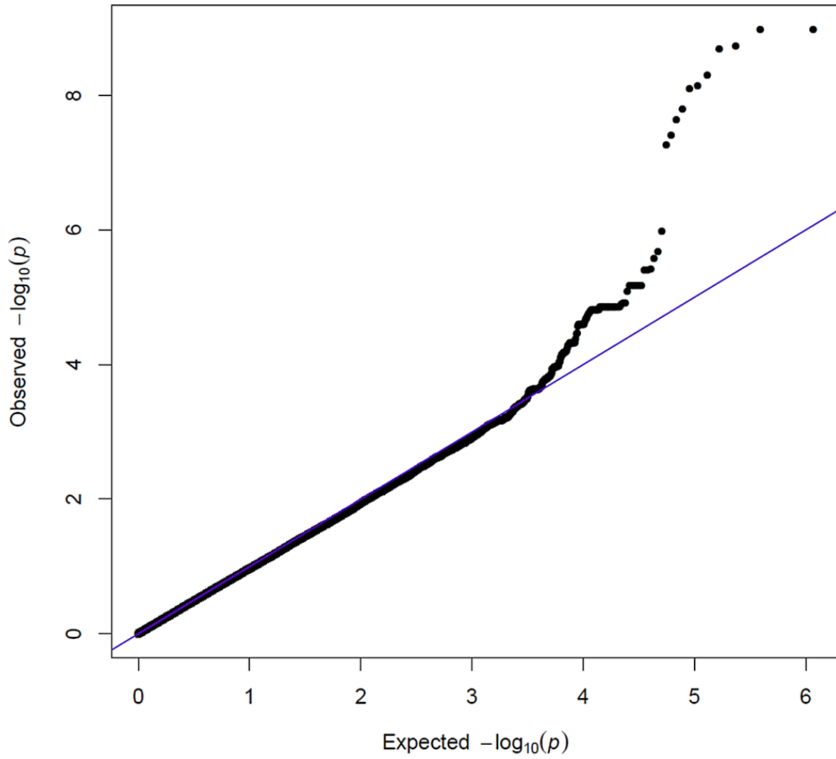
Figure S1. Q-Q plot of p-values for the GWAS of RFI.
