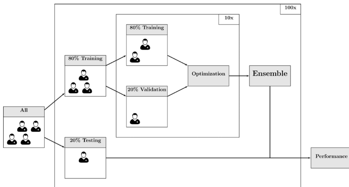
Figure S1. Visualization of the 100x stratified random-split cross-validation, including a second cross-validation within the training set to perform the automatic workflows optimization. Optimization was done solely on the training set in order to prevent overfitting on the test set. The ensemble averages the predictions of the best 50 performing workflows to create a more robust model.
