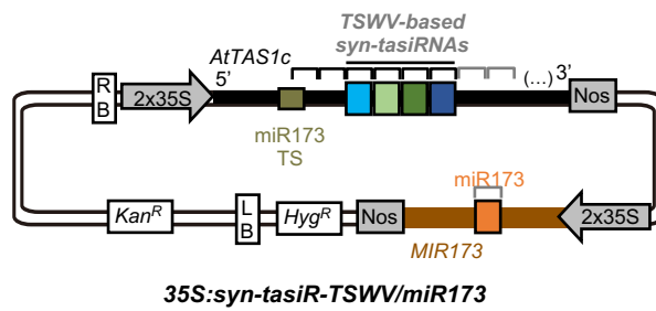
Figure S1. Diagram of the complete 35S:syn-tasiR-TSWV/miR173 plasmid. Approximate locations of T-DNA right and left borders (RB and LB, respectively) as well as bacterial and plant antibiotic resistance genes (kanamycin and hygromycin, respectively) are indicated. Other details are described in Figure 1a.
