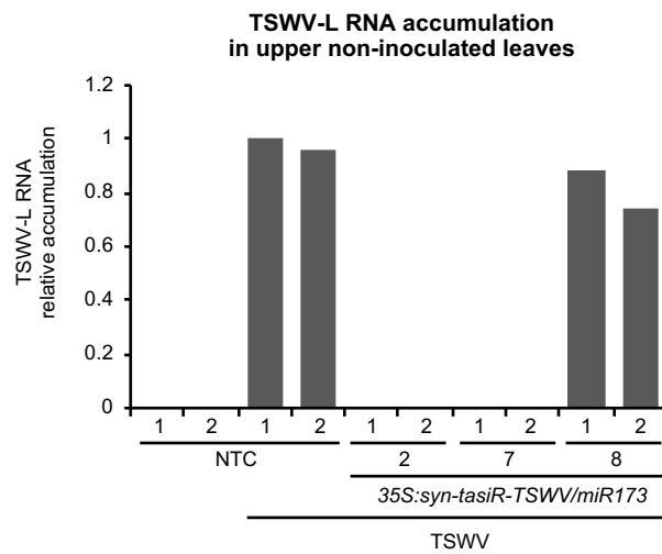
Figure S3. Relative TSWV-L RNA accumulation at 40 dpi in selected syn-tasiRNA lines and non-transgenic controls (NTCs) after normalization to Solanum lycopersicum actin ( Tom41 ) and Elongation Factor 1 alpha ( eEF1a ), as determined by RT-qPCR (NTC infected plant 1 = 1.0).
