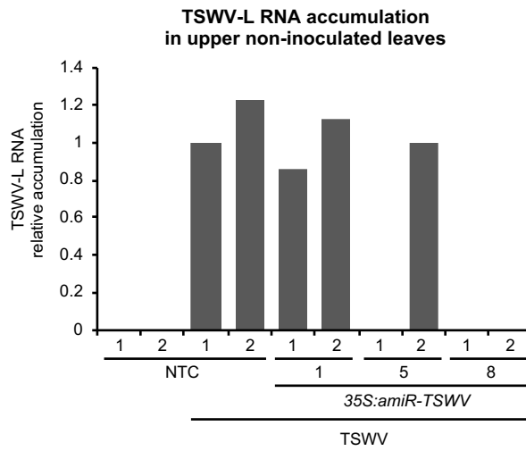
Figure S5. Relative TSWV-L RNA accumulation at 40 dpi in selected amiRNA lines and non-transgenic controls (NTCs) after normalization to Solanum lycopersicum actin ( Tom41 ) and Elongation Factor 1 alpha ( eEF1a ), as determined by RT-qPCR (NTC infected plant 1 = 1.0).
