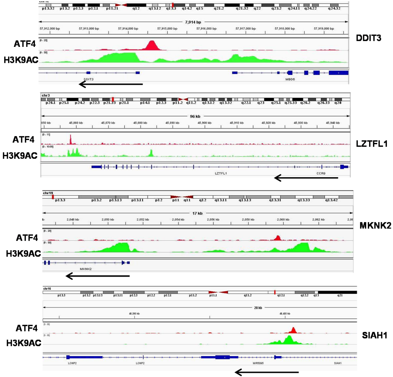
Figure S4. ChIP -seq profiles of ATF4 target genes (DDIT3, MKNK2, LZTFL1, SIAH1) and H3K9Ac in MZCRC1 cells treated with eeyarestatin. The peaks represent sequences bound by ATF4 and H3K9Ac. Arrows indicate the direction of transcription.
