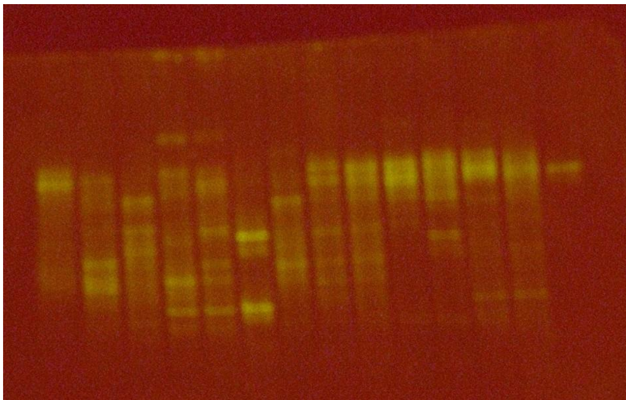
S1 Fig. Raw original image of bacterial DGGE profiles of the DNA extracted directly from the analysed samples and amplified with primers 338fGC and 518r
