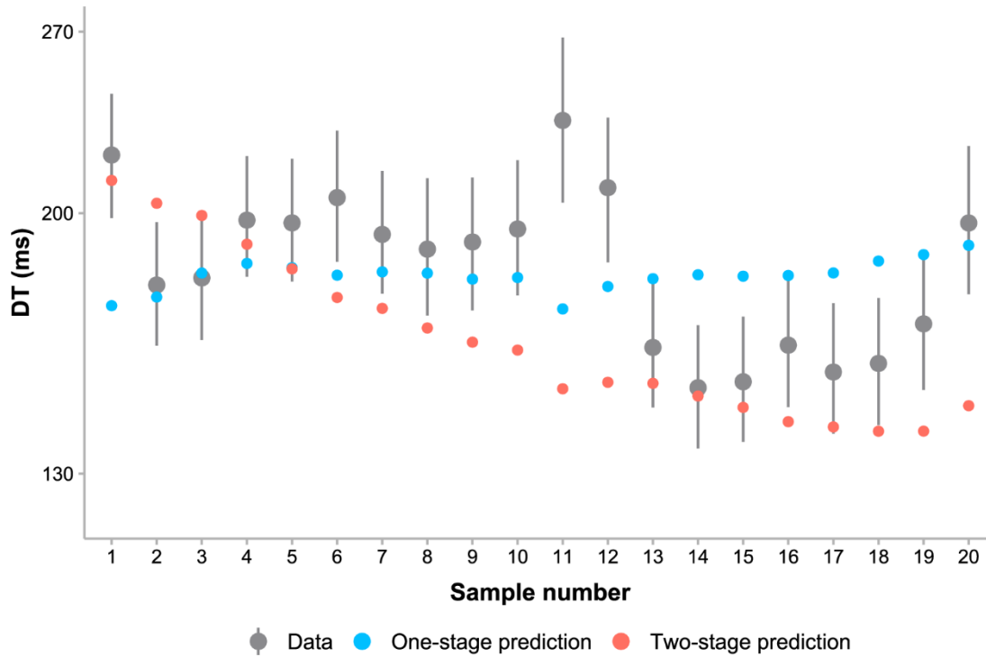
S4 Fig. Decision time as a function of sample number: data vs. model predictions. The observed decision times had a significant decreasing trend with the increase of sample number ( t = -12.26, p < .001 ), which was captured by the best two-stage model (red dots) but not by the best one-stage model (blue dots).
