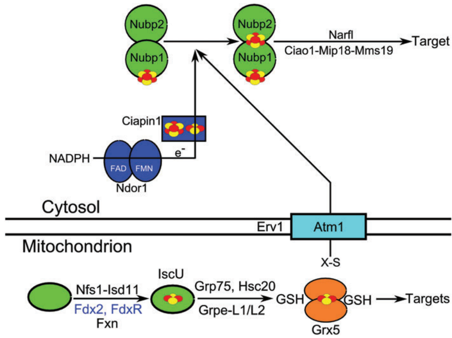
SUPPLEMENTARY FIG. S5. Illustration of Fe/S synthesis machinery in mammals. This figure was adapted from Lill et al. (25). X-S represents the sulfur-containing moiety exported from the mitochondria, and sulfur and iron atoms are represented in yellow and red , respectively. Scaffold proteins are shown in green and proteins involved in electron transport in blue . Fe/S, iron-sulfur cluster.
