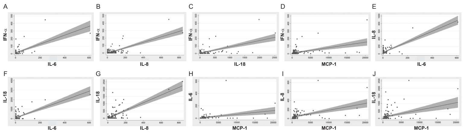
Fig. S2 The correlation between each cytokine in all SLE patients (N=124) The correlation coefficient were shown in Table 3.
