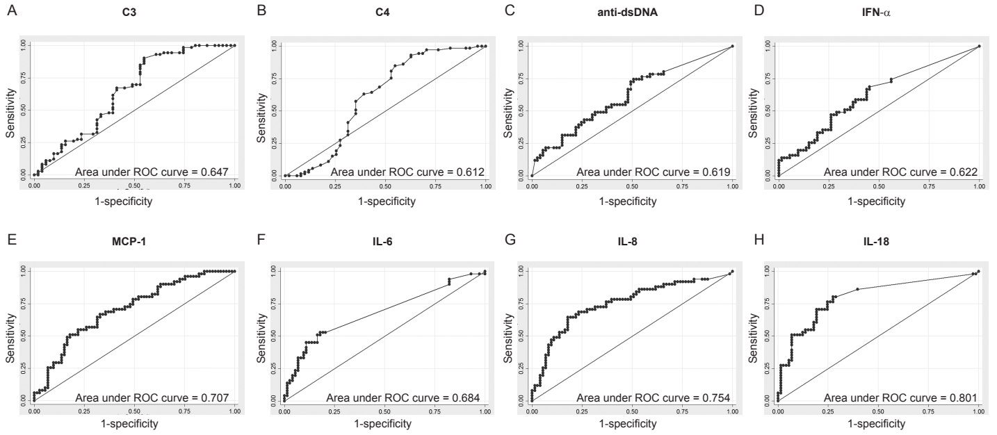
Fig. S3 Receiver operating characteristic (ROC) curve and area under ROC curve in SLE patients (N=124). The following biomarkers of C3 (A), C4 (B), anti-dsDNA (C), IFN- \alpha (D), MCP-1 (E), IL-6 (F), IL-8 (G), and IL-18 (H) were showed.
