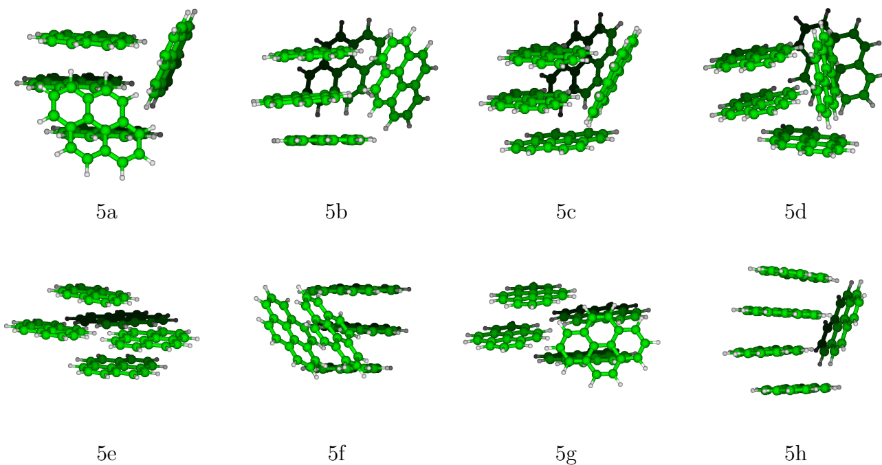
Figure S4: most stable structures for neutral pyrene pentamer
