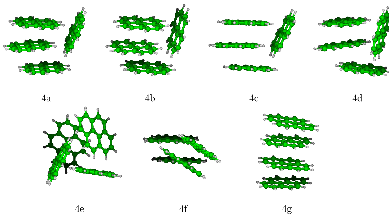
Figure S3: most stable structures for neutral pyrene tetramer
