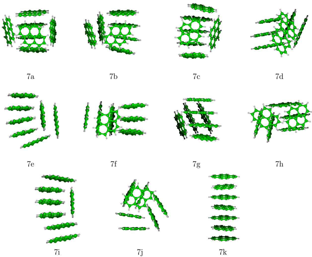
Figure S12: most stable structures for cationic pyrene heptamer
