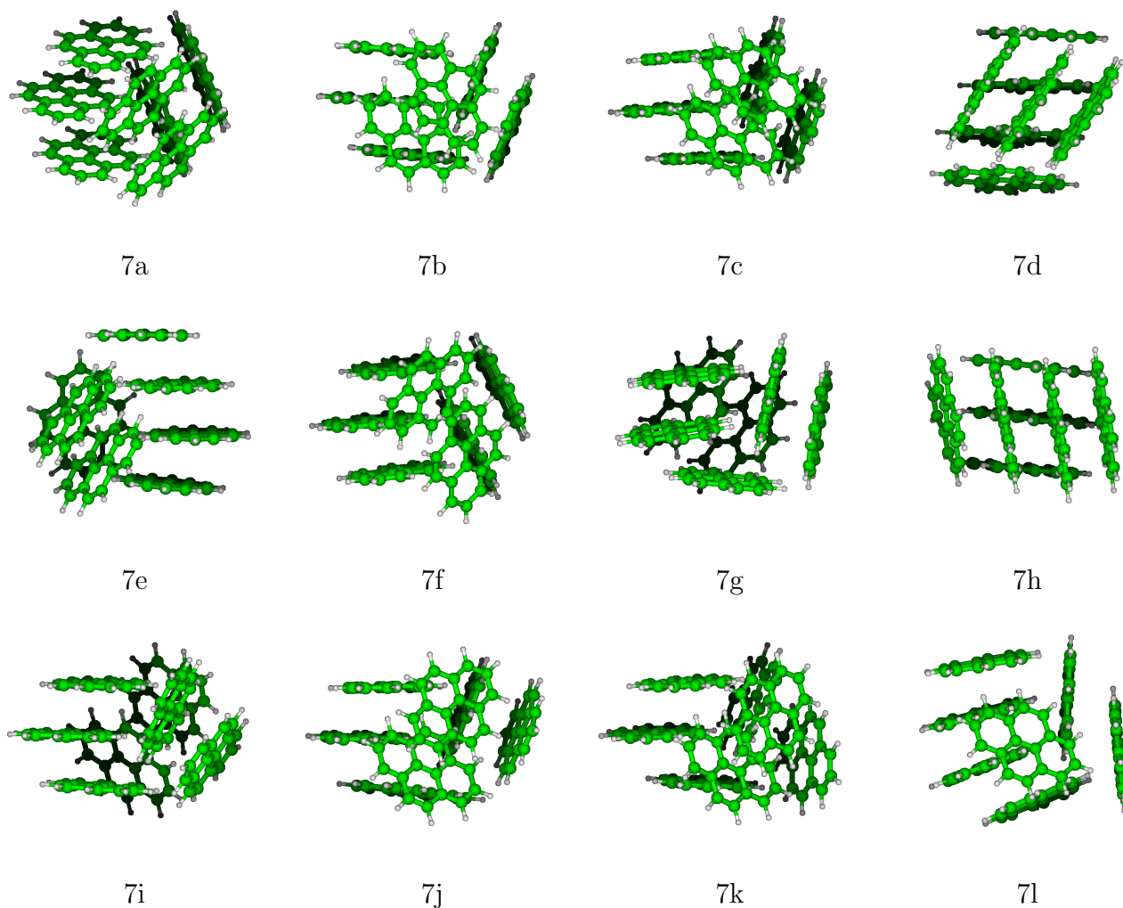
Figure S6: most stable structures for neutral pyrene heptamer
