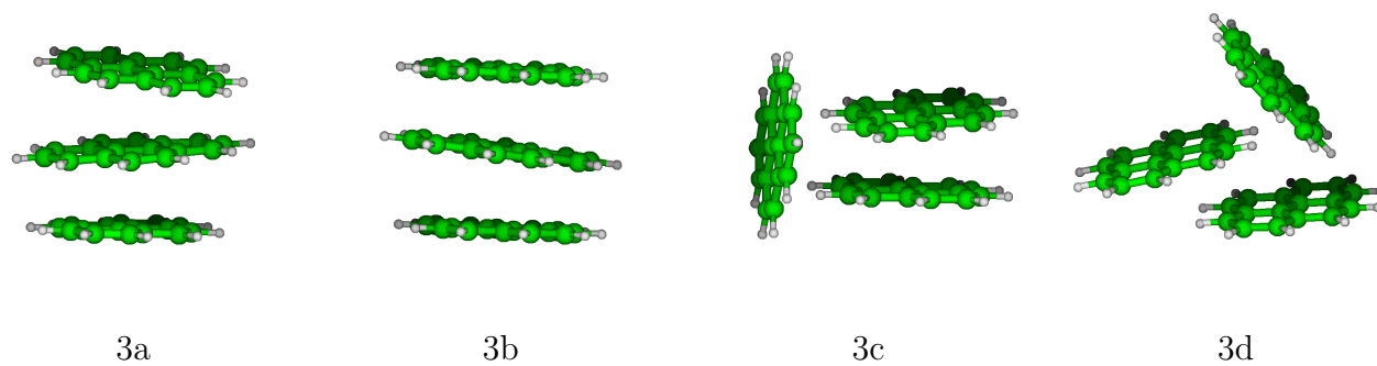
Figure S8: most stable structures for cationic pyrene trimer
