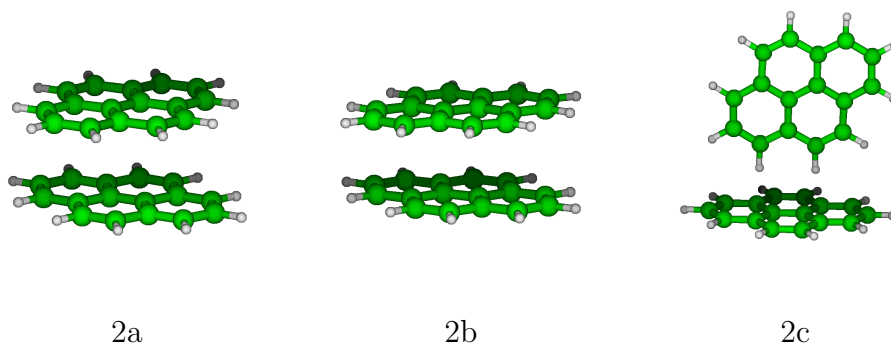
Figure S1: most stable structures for neutral pyrene dimers
