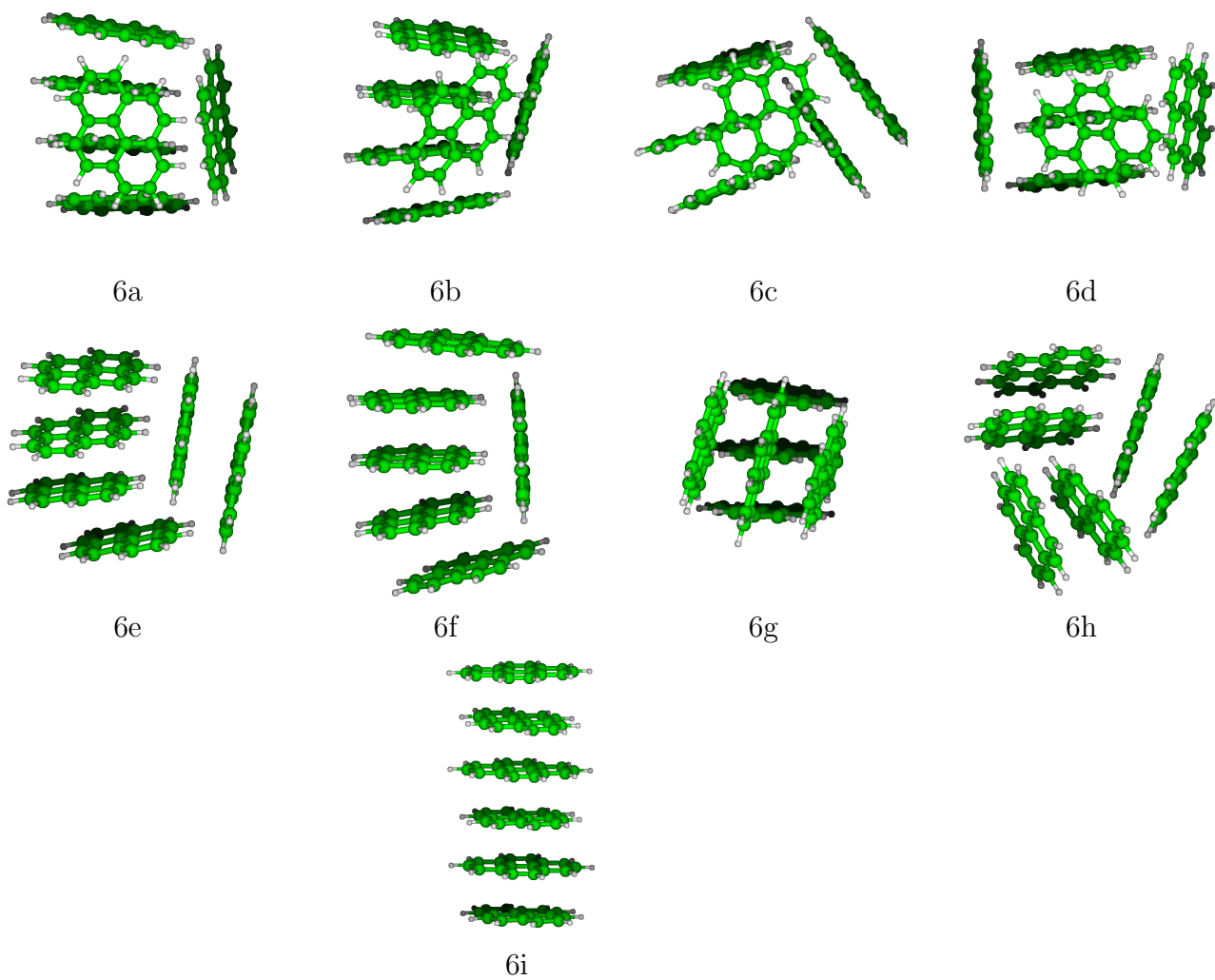
Figure S11: most stable structures for cationic pyrene hexamer
