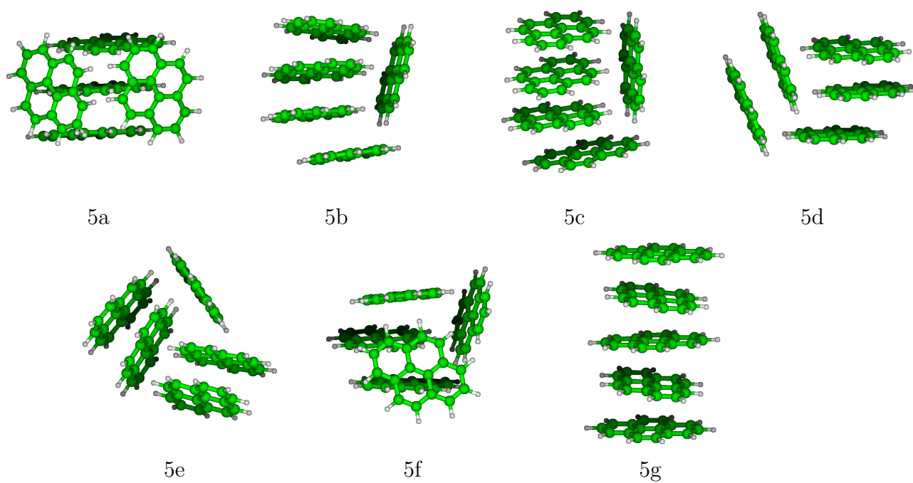
Figure S10: most stable structures for cationic pyrene pentamer
