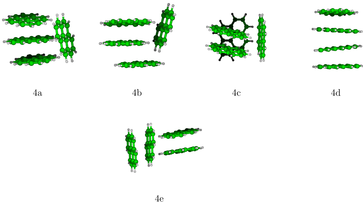
Figure S9: most stable structures for cationic pyrene tetramer
