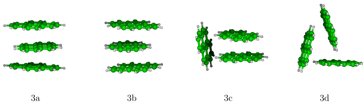
Figure S2: most stable structures for neutral pyrene trimer
