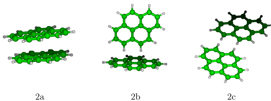
Figure S7: most stable structures for cationic pyrene dimers
