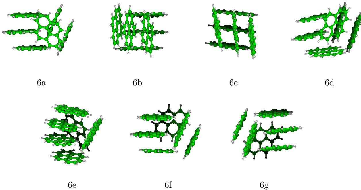
Figure S5: most stable structures for neutral pyrene hexamer
