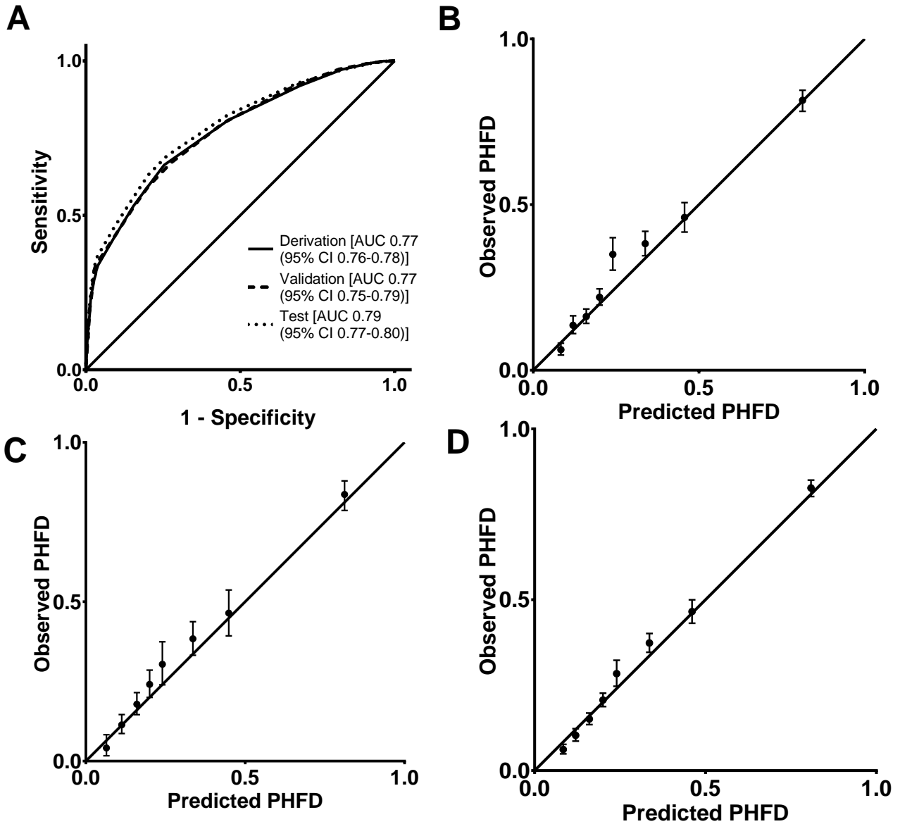
Supplemental Figure 2. Receiver operator characteristic (ROC) curves of risk score model for post hip fracture delirium (PHFD) in derivation and validation cohorts (A). Calibration plots showing observed and predicted PHFD risk across the range of risk scores (0-20) for derivation (B), validation (C) and test cohorts (D).
