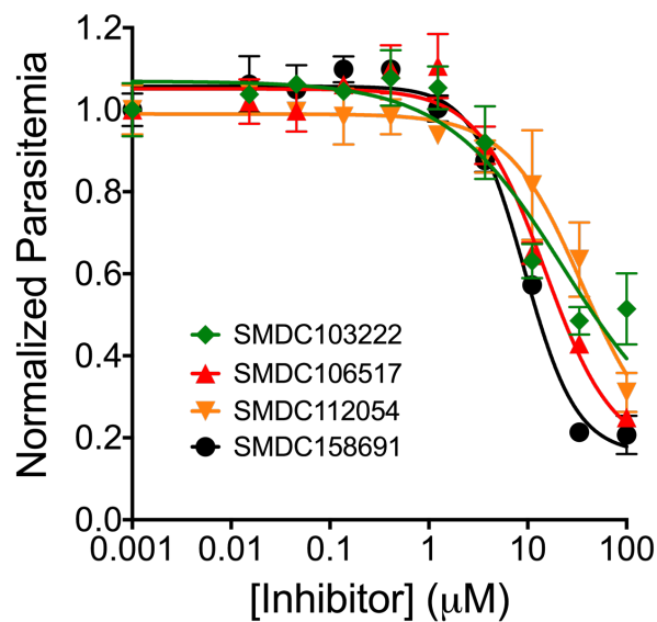
S1 Figure. Antiparasitic activity of selected hits. A synchronized culture of P. falciparum at 1% parasitemia and 1% haematocrit was treated at ring stage with different concentrations of the indicated compounds and cultured for 72 h. Samples were then fixed, the iRBCs stained with propidium iodide, and the parasitemia quantified by flow cytometry. Normalized parasitemia relative to DMSO controls is shown. \text{EC}_{50} values are reported in Tables 1 and 2.
