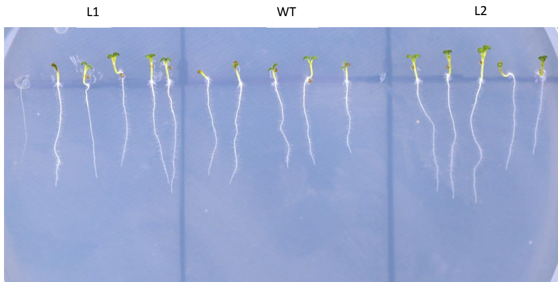
Figure A: The root growth experiment directly on MS medium. The left in the panel is L1, the middle is WT, and the right is L2.
