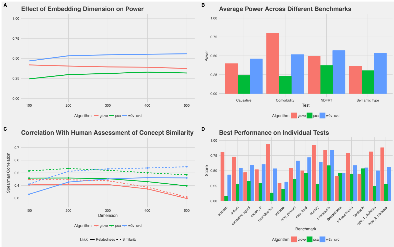
Supplemental Figure 1: Results on combined data. Panel A: The effect of embedding dimension on statistical power, averaged across benchmarks. Panel B: Power for the best configuration for each algorithm across each benchmark category (standard errors show as black bars). Panel C: The effect of embedding dimension on spearman correlation between concept-concept cosine similarity with human assessments of similarity and relatedness. Panel D: Best performance by each algorithm on individual tests.
