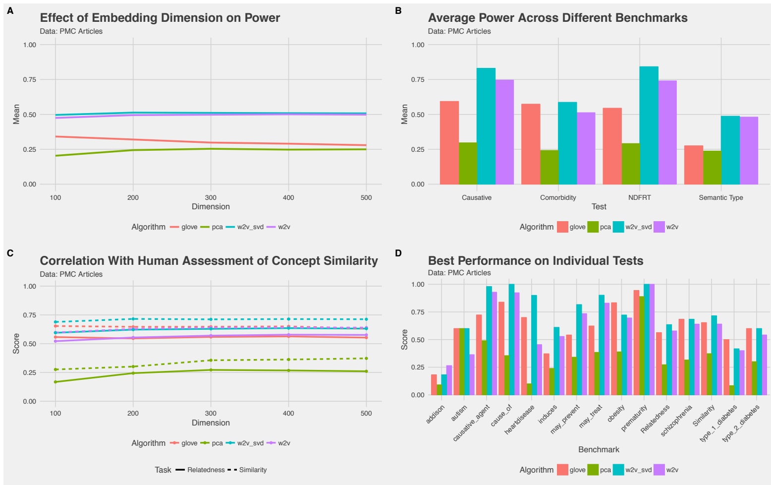
Supplemental Figure 3: Results for GloVe, PCA, and word2vec (SVD and original as implemented in the genism package) on the full text articles from PubMed.
