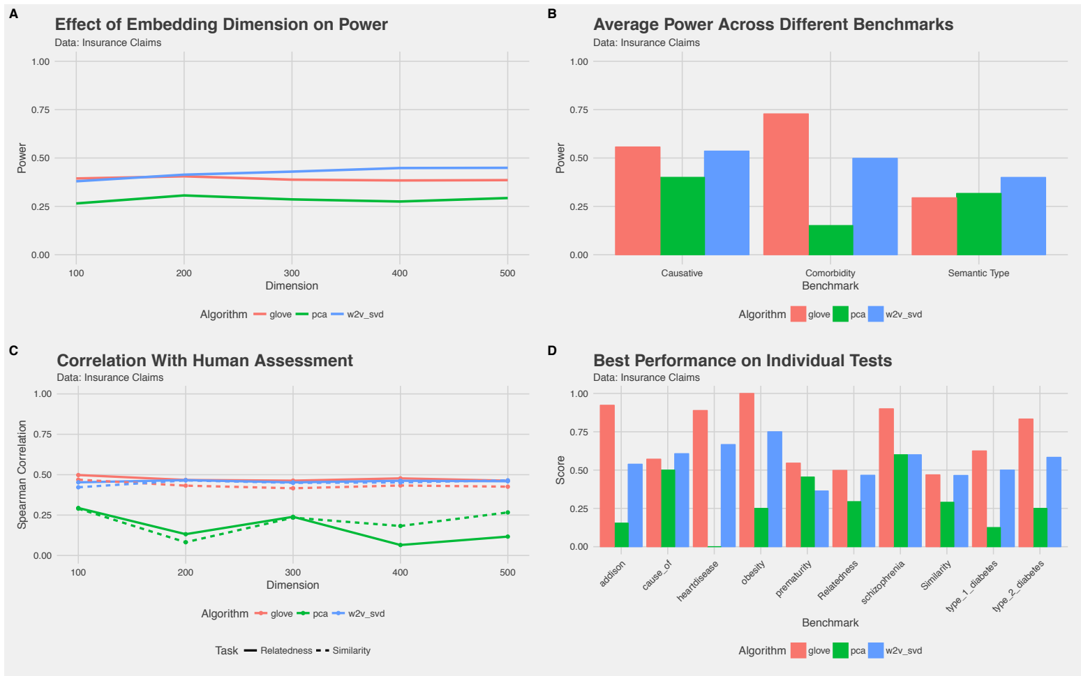
Supplemental Figure 2: Results for GloVe, PCA, and word2vec on the insurance claims data.
