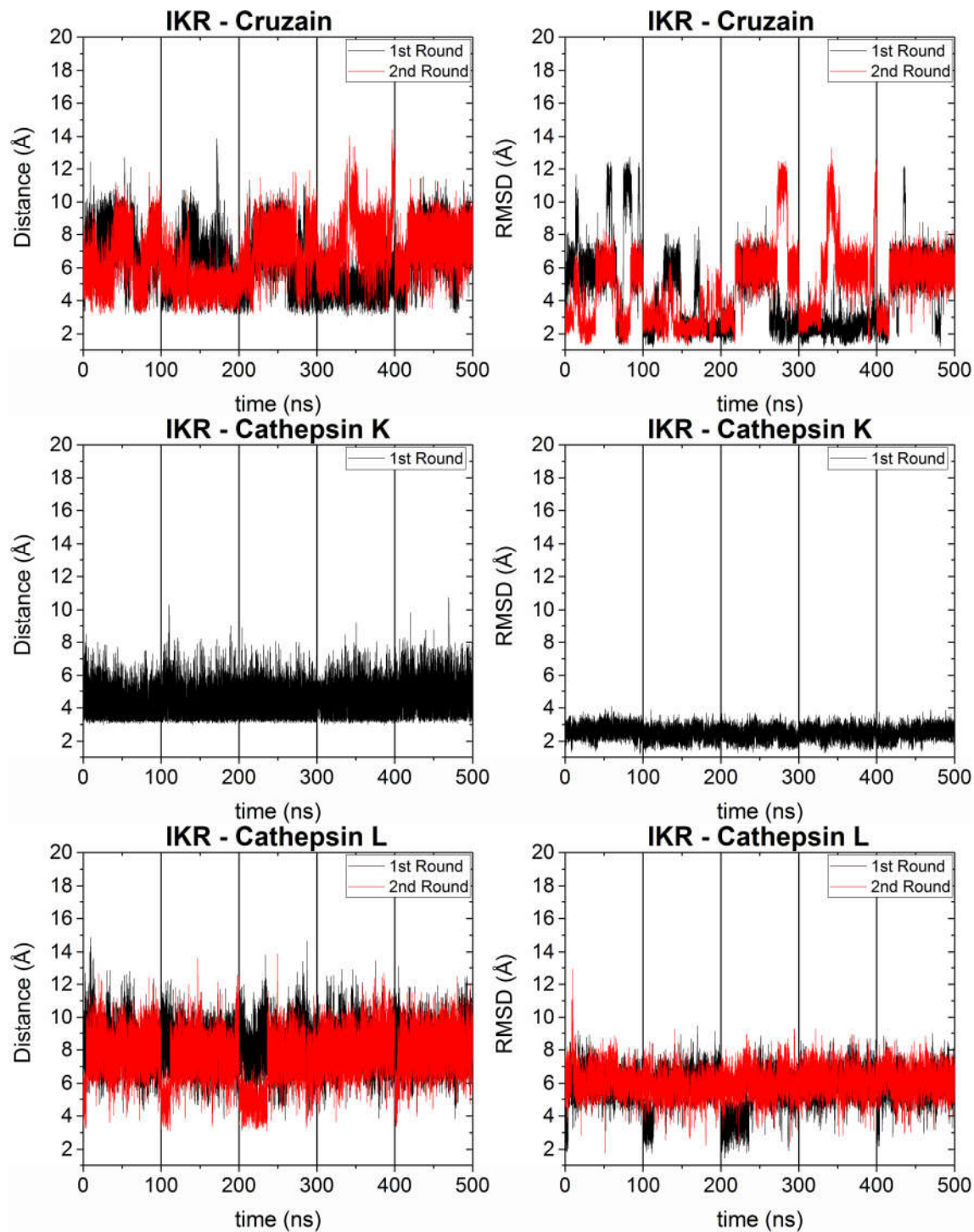
Figure S 4 Distance between IKR nitrile and sulfur from Cys25 residue (first column) e RMSD of IKR ligand (second column) complexed with cruzain, cathepsin K and cathepsin L (first, second and third row respectively). Black vertical bars delimit the replicates. Black and red lines represent respectively Round 1 and 2 simulations.
