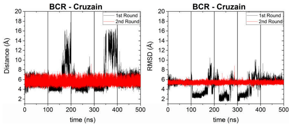
Figure S 5 - Distance between BCR nitrile and sulfur from Cys25 residue (first column) e RMSD of the ligand (second column) complexed with cruzain. Black vertical bars delimitate the replicates. Black and red lines represents respectively Round 1 and 2 simulations.
