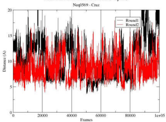
Distance between C#N and Cys25
