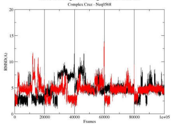
RMSD of ligand during MD simulation
