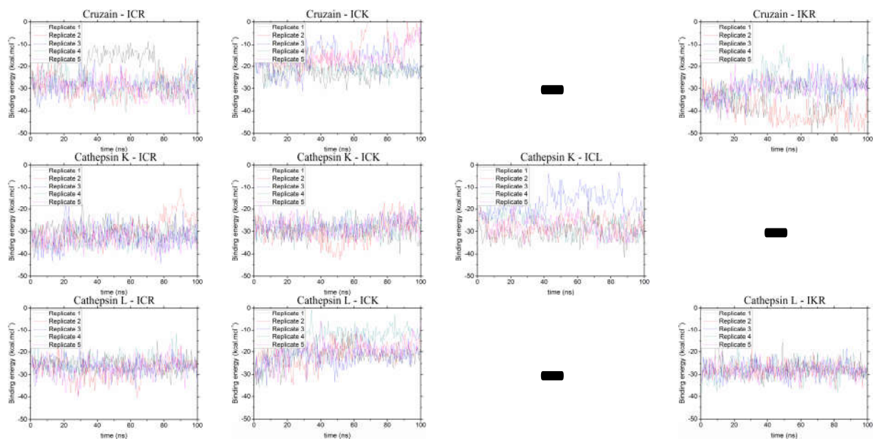
Figure S 8 - Binding free energy over the time of Round 2 of simulations for ligands ICR, ICK, ICL and IKR (first, second, third and fourth column respectively) complexed with cruzain (first row), cathepsin K (second row) and cathepsin L (third row). Different colors represented different replicates of the same system
