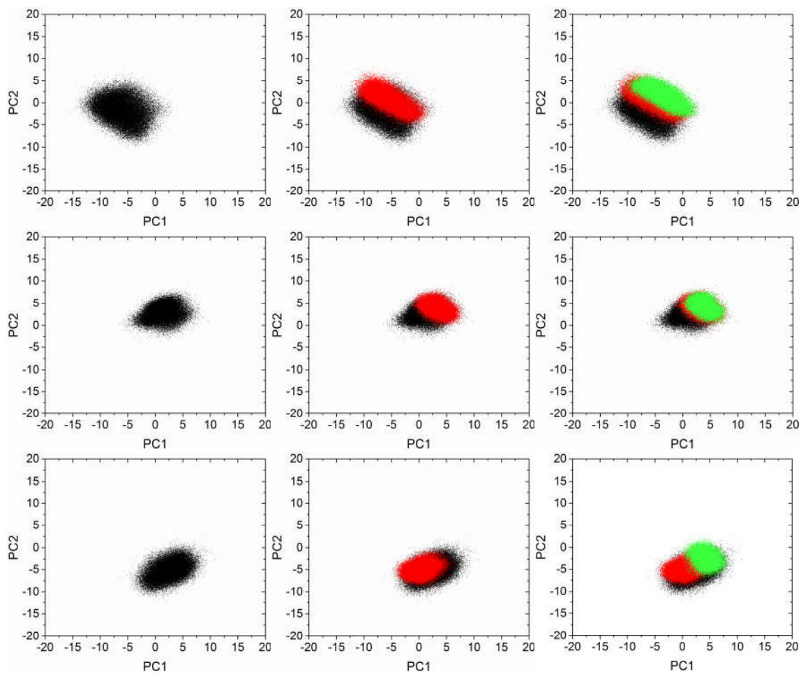
Figure S 9 - Projection over the first two principal components of cruzain (first row), cathepsin K (second row) and cathepsin L (third row) simulation frames in its apo form and complexed with noncovalent and covalent forms of ligand ICR (black, red and green dots, respectively).
