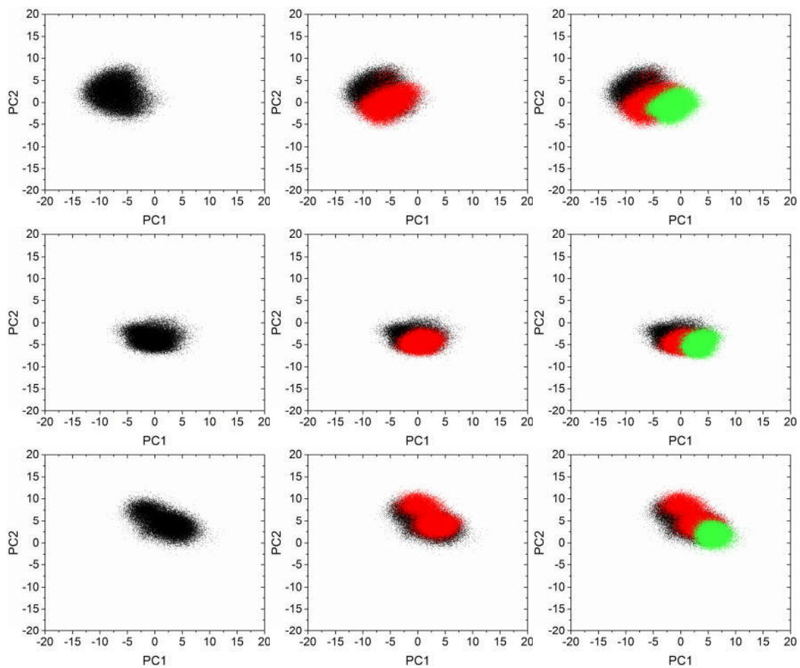
Figure S 10 - Projection over the first two principal components of cruzain (first row), cathepsin K (second row) and cathepsin L (third row) simulation frames in its apo form and complexed with noncovalent and covalent forms of ligand ICK (black, red and green dots, respectively).
