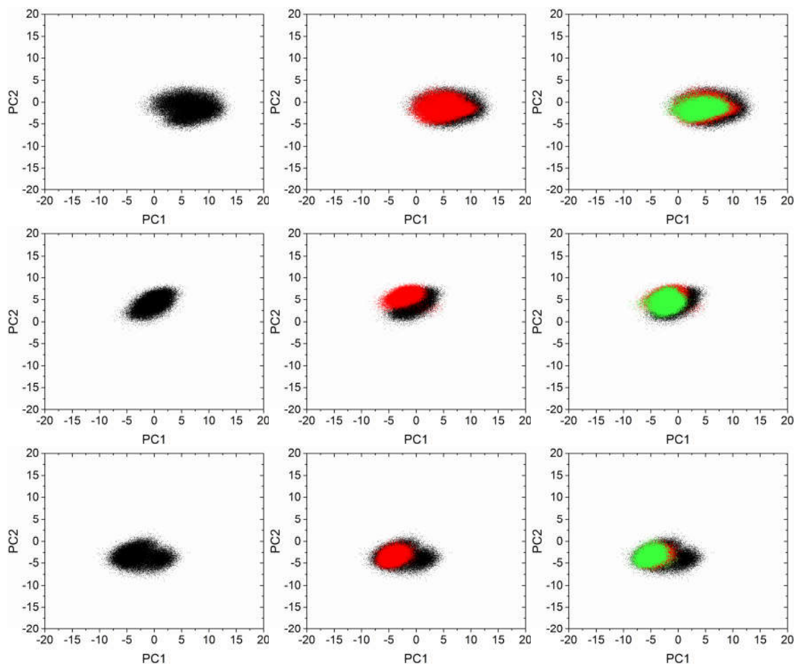
Figure S 11 - Projection over the first two principal components of cruzain (first row), cathepsin K (second row) and cathepsin L (third row) simulation frames in its apo form and complexed with noncovalent and covalent forms of ligand ICL (black, red and green dots, respectively).
