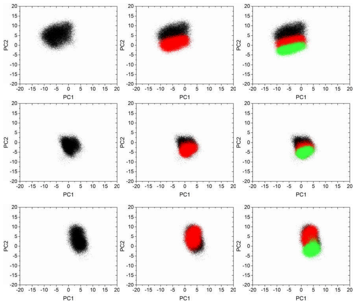
Figure S 12 - Projection over the first two principal components of cruzain (first row), cathepsin K (second row) and cathepsin L (third row) simulation frames in it apo form and complexed with noncovalent and covalent forms of ligand IKR (black, red and green dots, respectively).
