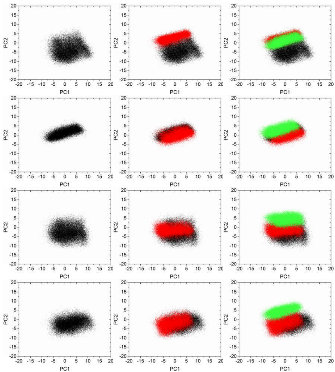
Figure S 13 - Projection over the first two principal components of cruzain simulation frames in it apo (black dots) form and complexed with noncovalent (red dots) and covalent forms (green dots) of ligands Neq0409 (first row), Neq0544 (second row), Neq0569 (third row) and Neq0568 (fourth row).
