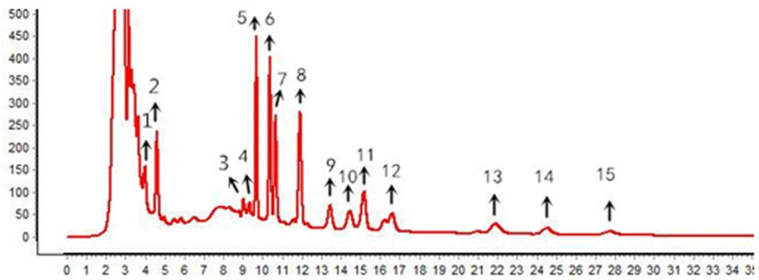
Fig 1. The HPLC fingerprint of YPFS decoction
