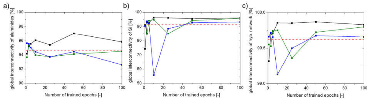
Supplementary figure 1 - Global interconnectivity of Si, aluminides and the hybrid Si+aluminides networks
