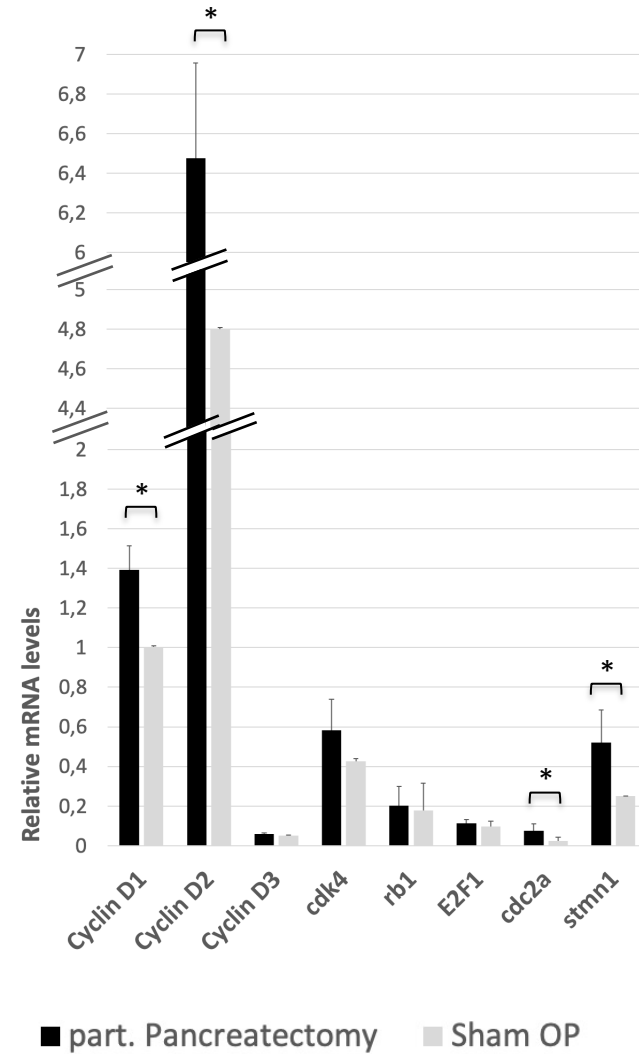
Figure 3: Gene expression signal following affymetrix hybridization of RNA extracted from islets isolated by LCM from sham operated (grey bars) or pancreatectomized (black bars) mice: (a) on genes that were differentially expressed in Min6 cells overexpressing miR-132 and (b) on selected genes known for their role on cell proliferation and cell cycle.
