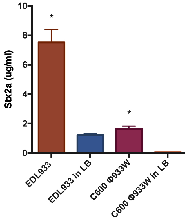
Fig. S1: EDL933 and C600 carrying φ933W were grown in 0.1229 cell-free supernatant, or in LB as indicated. One-way ANOVA was used and levels marked with an asterisk were significantly higher than respective LB control (Dunnett's test, p < 0.05 ).
