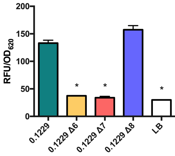
Fig. S3: W3110Δ tolC PrecA-gfp was grown with 0.1229 and 0.1229 regional (A) or individual ORF (B) knockouts, or alone indicated by LB. One-way ANOVA was used and levels marked with an asterisk were significantly lower than 0.1229 (Dunnett's test, p < 0.05 ).
