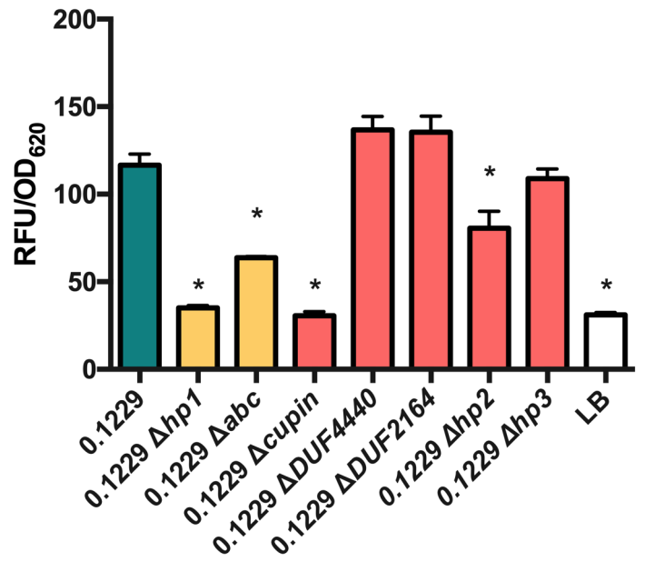
Fig. S3: W3110Δ tolC PrecA-gfp was grown with 0.1229 and 0.1229 regional (A) or individual ORF (B) knockouts, or alone indicated by LB. One-way ANOVA was used and levels marked with an asterisk were significantly lower than 0.1229 (Dunnett's test, p < 0.05 ).
