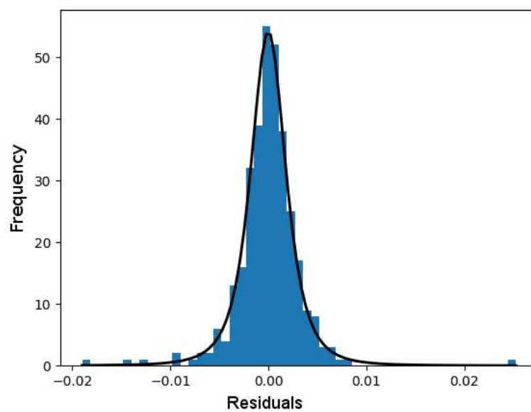
Figure S1: A histogram (blue) showing the distribution of amide proton chemical shift residuals in the example data (from all residues for which curvature is not detected, at all temperatures). A t distribution (black line) fit to these residuals is superimposed.
