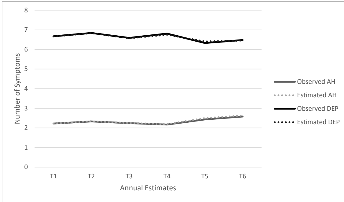
Figure 1. Estimated and actual anhedonia (AH) and depressed mood (DEP) means from the Center for Epidemiological Studies Depression (CESD-10) scale. Estimated means were derived from a latent growth curve model using Mplus version 7.2.
