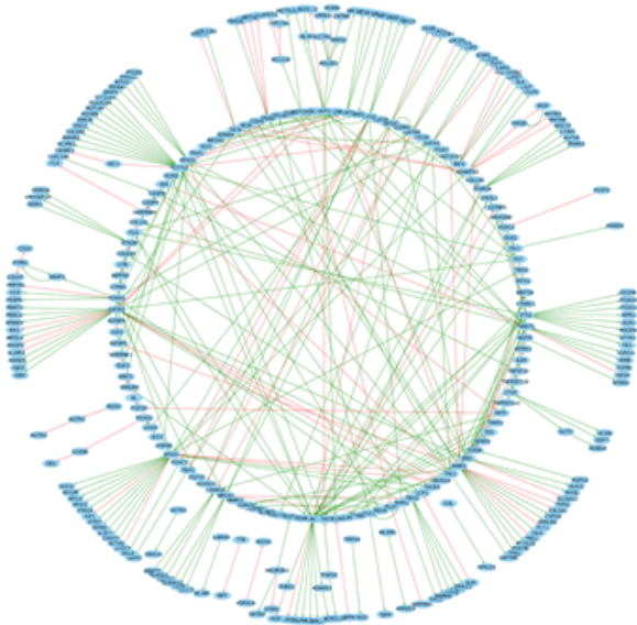
a Control gene regulatory network
