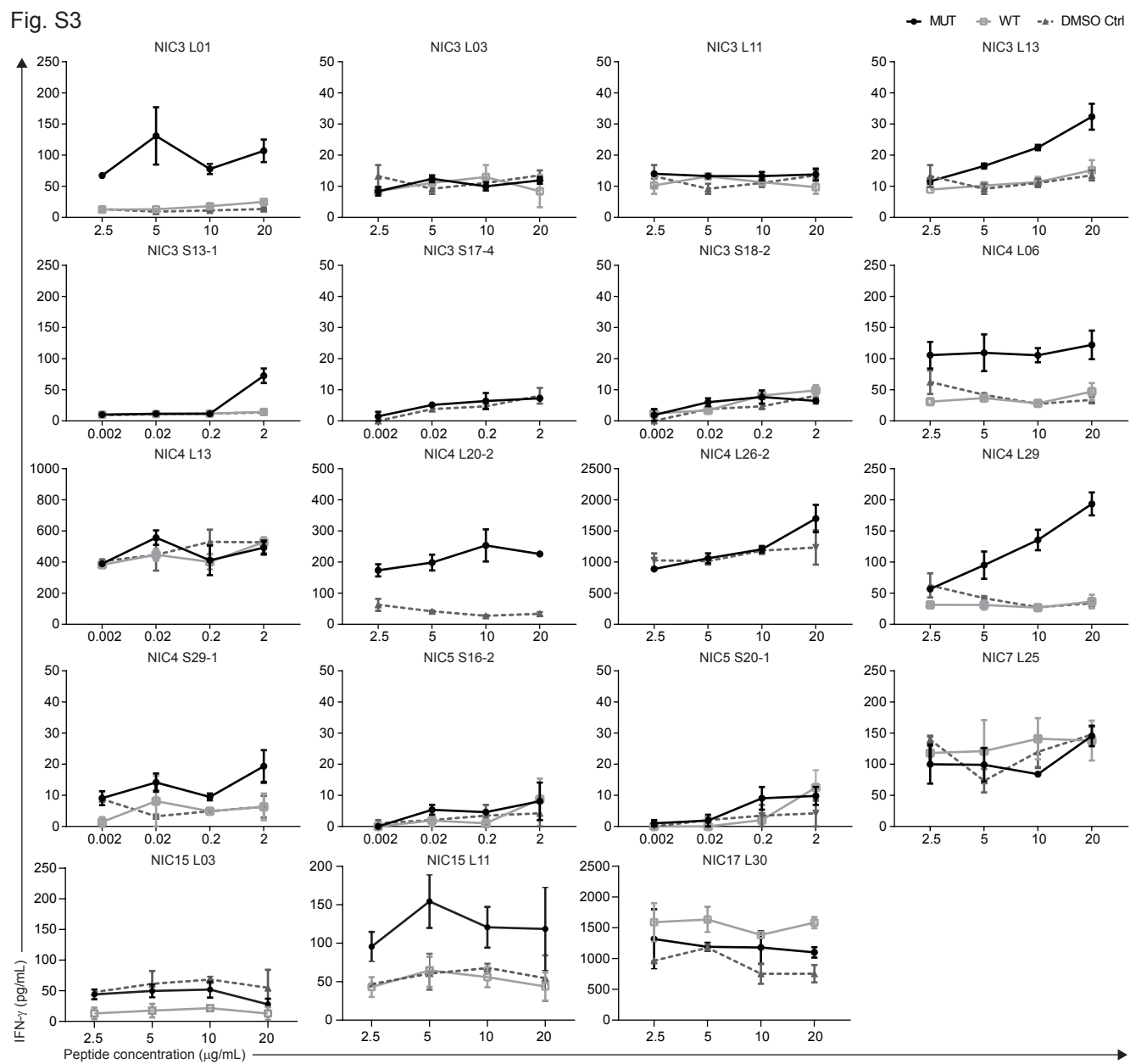
Figure S3 | Validation of the neoantigen-specific responses detected in the first screen. IFN- \gamma production of TIL and PBL from NIC3-7, NIC15 and NIC17 was measurement upon stimulation with mutant (black) and wild type (grey) HPLC peptides, and a DMSO control (dashed), at different peptide concentrations. The mean \pm standard deviation of the biological duplicates in the same experiment are depicted.
