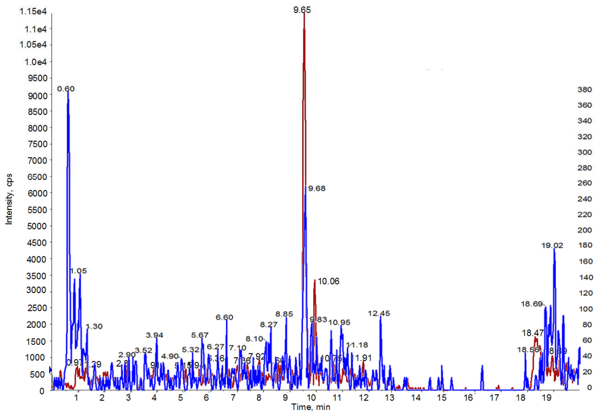
Supplemental Figure S2. of HPLC separated LTB 4 . Internal standard added to the sample prior extraction (red) and overlaid sample (blue). Left scale corresponds to the counts per second (cps) for internal standard and right for sample. Monitored ion pairs (MRM) were 339.1/130.1 amu for internal standard and 335.1/129.1 amu for EV sample.
