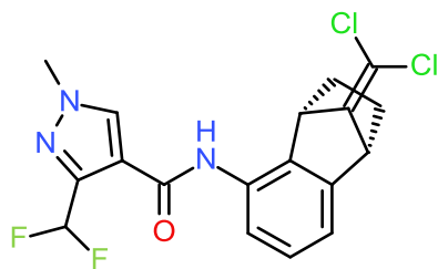
Benzovindiflupyr
