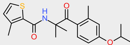
Isofetamid
