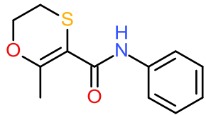
Carboxin
