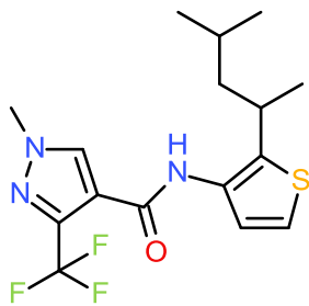
Penthiopyrad
