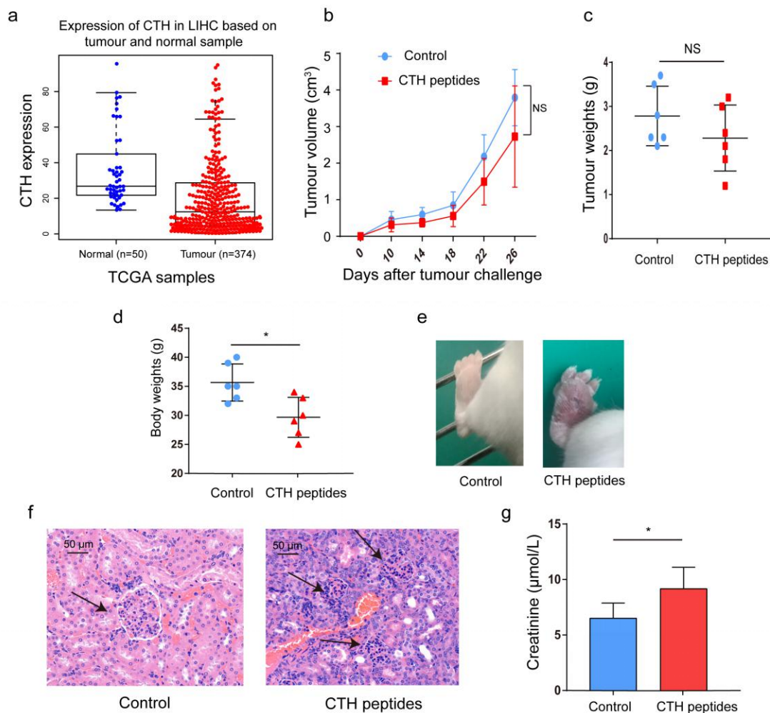
Supplementary Fig. 2 The efficacy and side-effects of CTH peptides. (a) Expression of CTH in liver hepatocellular carcinoma (n=374) and normal tissue (n=50) were analysed by TCGA database. (b) Growth curve of H22 hepatoma in control and CTH
