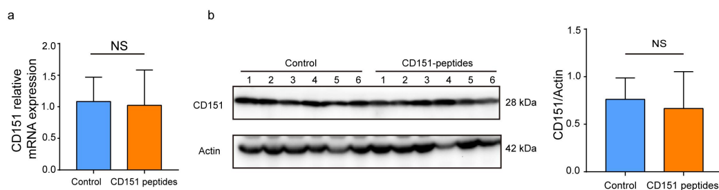
Supplementary Fig. 1 CD151 expression on the tumour cells after peptide vaccination. (a) MRNA expression of CD151 on the tumor cells after peptide vaccination (n=6/group); (b) protein expression of CD151 on the tumor cells after peptide vaccination (n=6/group). Results are representative of two independent experiments. P -values were determined by two-tailed Student's t-test (NS, P >0.05).
