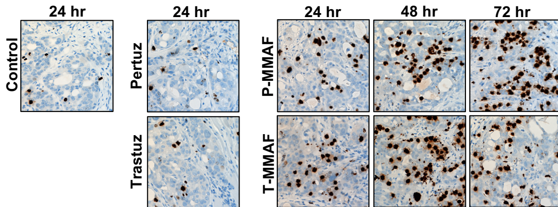
Supplementary Figure 5: MMAF anti-HER2 antibody conjugates increase tumor G 2 /M fraction. NCI N87 tumor bearing mice injected with 1 nmole of free antibodies or MMAF conjugates. Tumors harvested 24, 48 and 72 hours later and stained for G 2 /M marker pS10 histone H3.
