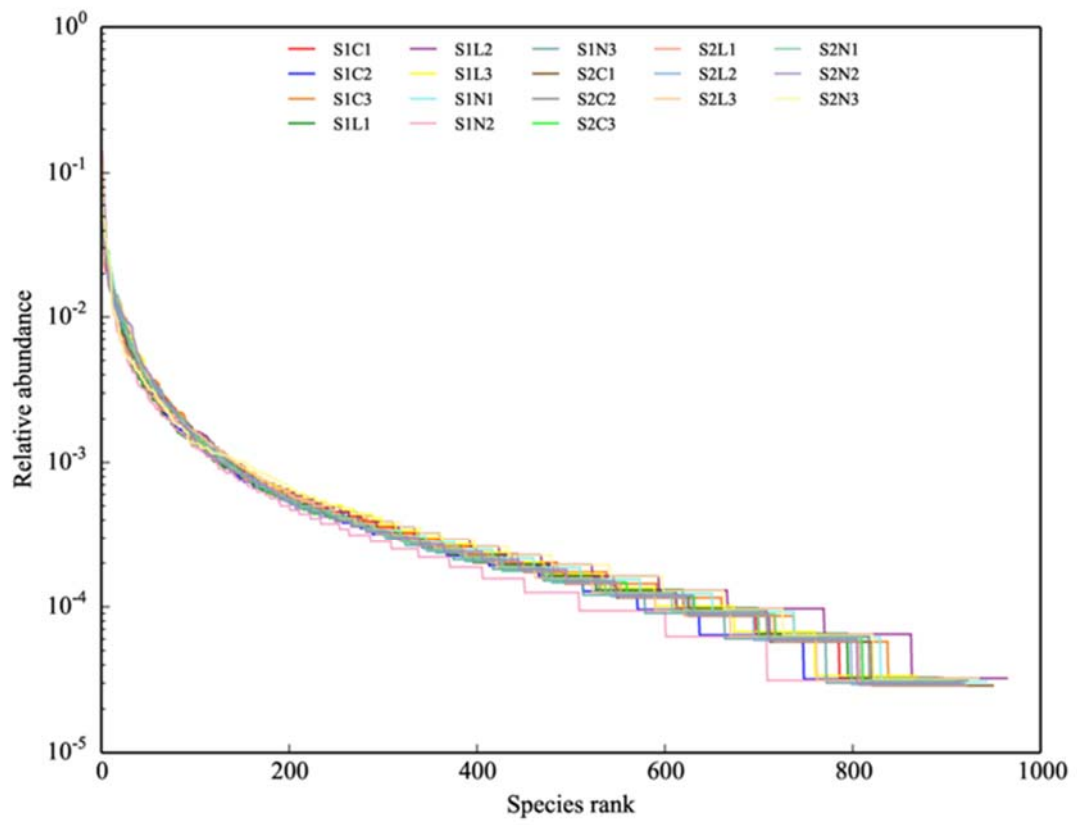
Supplementary Figure S6. Rank Abundance curve for all samples.
