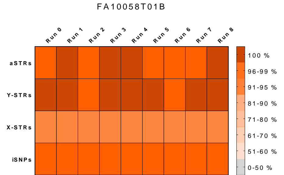
Figure S3. Ancient DNA heat maps for 27 autosomal STRs (aSTR), 24 Y-STRs, 7 X-STRs and 94 identity SNPs (iSNP) showing the percentage of concordantly typed forensic markers between all sequencing runs. Color gradient indicates the percentage of successfully typed alleles from 100% (intensive orange) down to \leq 50\% (light-grey), except for FA10013B01A. Color gradient for FA10013B01A indicates the percentage of successfully typed alleles 1-3% (light-grey) and drop-out (white).
