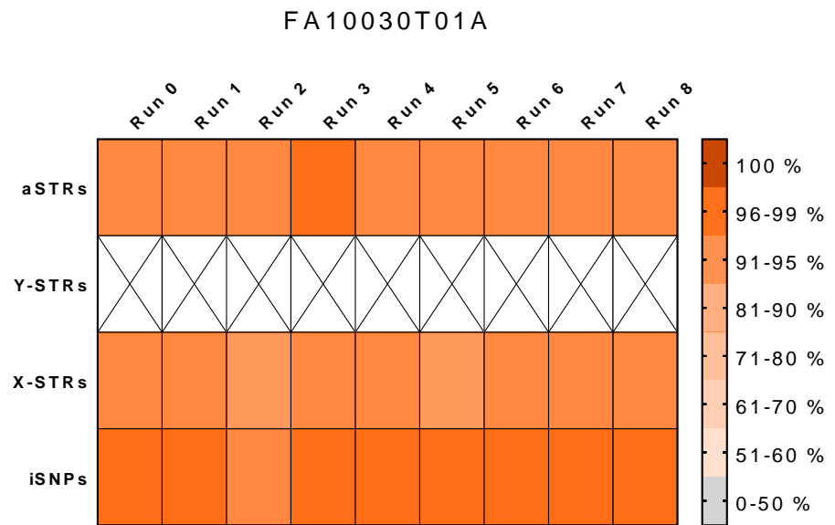
Figure S3. Ancient DNA heat maps for 27 autosomal STRs (aSTR), 24 Y-STRs, 7 X-STRs and 94 identity SNPs (iSNP) showing the percentage of concordantly typed forensic markers between all sequencing runs. Color gradient indicates the percentage of successfully typed alleles from 100% (intensive orange) down to \leq 50\% (light-grey), except for FA10013B01A. Color gradient for FA10013B01A indicates the percentage of successfully typed alleles 1-3% (light-grey) and drop-out (white).
